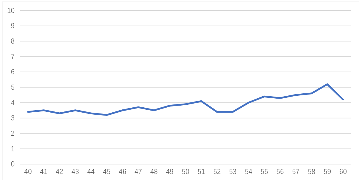
NF vs Frequency
